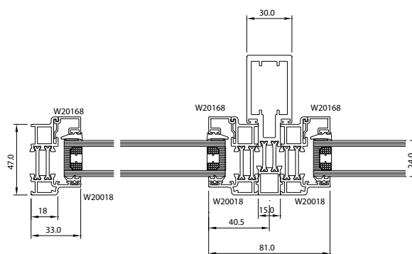
Horizontal section through fixed panes
