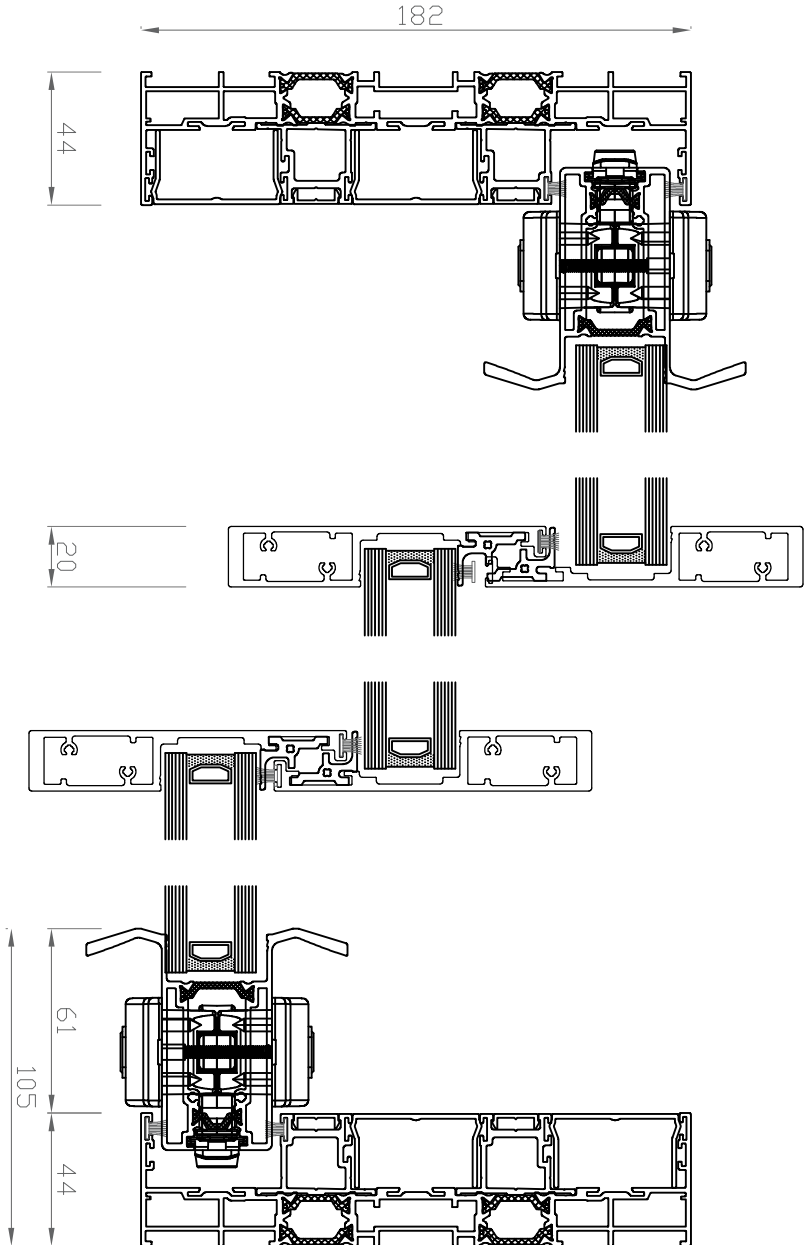
Horizontal cross section
