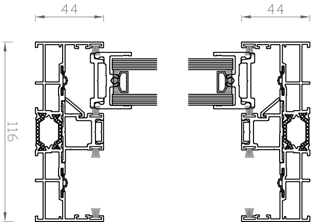
Double track sliding door Vertical cross section
