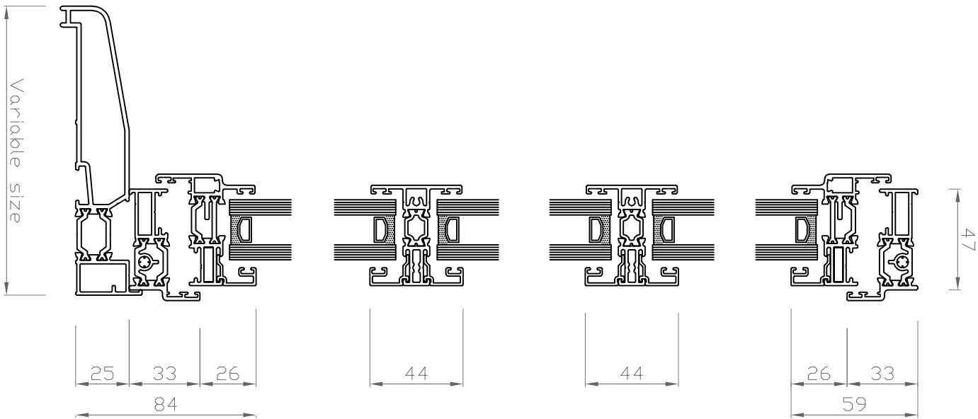
Vertical cross section
