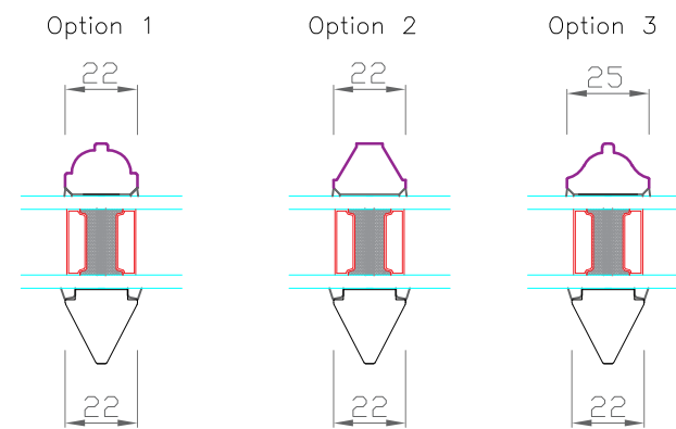
Stick on bars and internal bead moulding cross section
