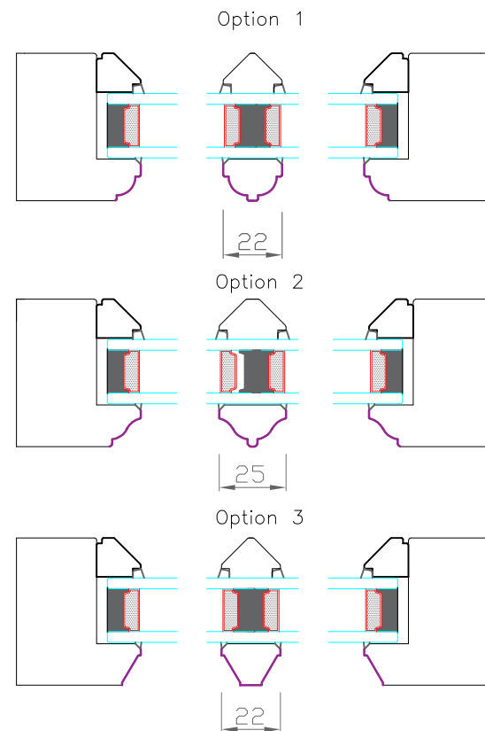
Glazing bead and stick on bars moulding cross section
